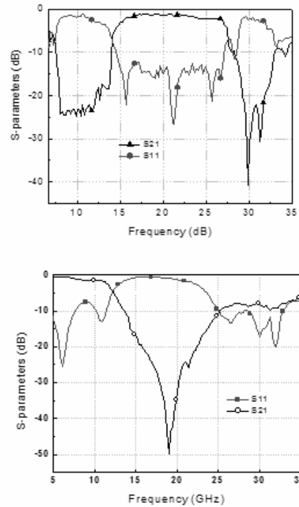
Fig. 21. Measurement results of the reconfigurable filter using MEMS switches (a) off-state of switch, band-pass filter and (b) on-state of switch, band-stop filter.
