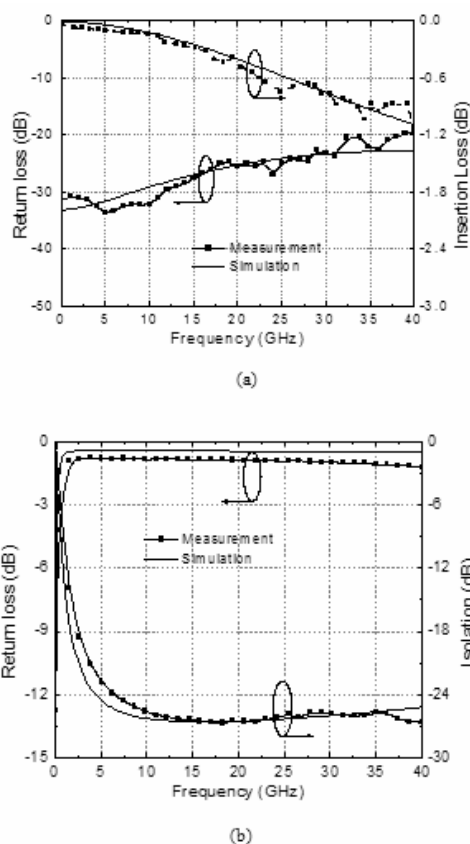
Fig. 11. Measurement and curve-fitted results (a) up-state; (b) down-state.
