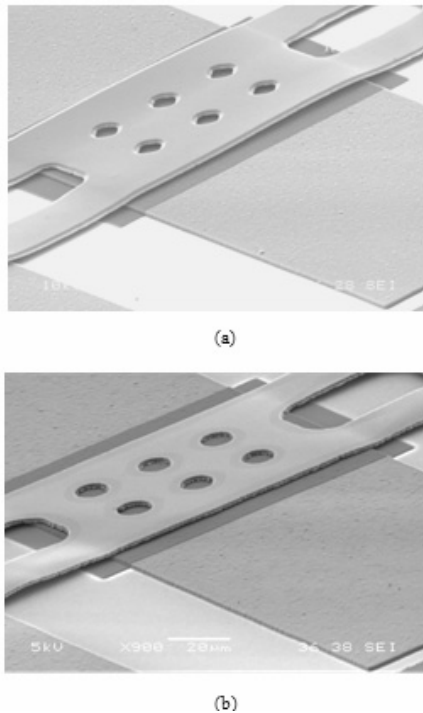
Fig. 7. SEM photos of the capacitive shunt switch. (a) Switch A, without fill-in photoresist and (b) Switch B, with fill-in photoresist.
