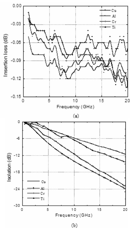
Fig. 9. Measurement results of RF properties versus different metal materials (a) insertion loss; (b) isolation (with applied hold-down voltage of 30 V).
