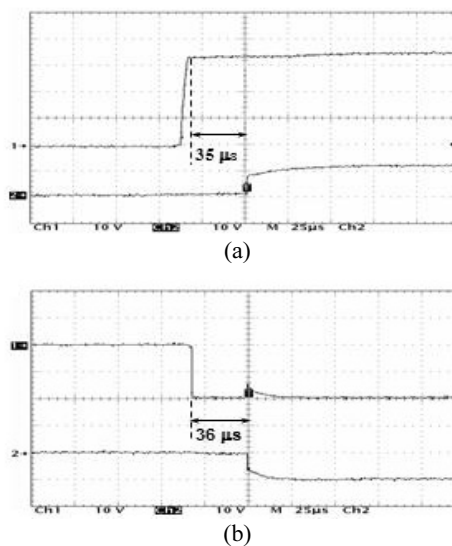
Fig. 5. Experimental results of switching performance of a lateral switch (a) close-state; (b) open-state.
