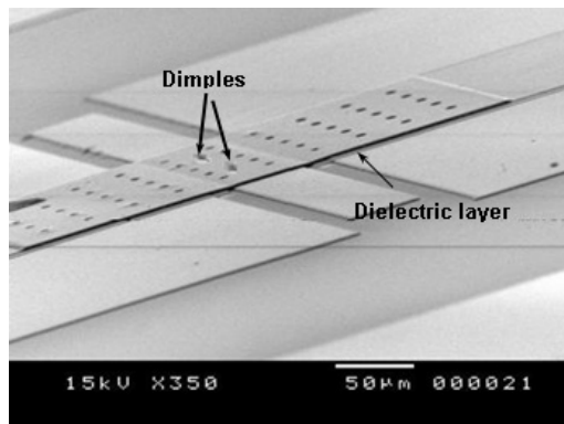
Fig. 10. SEM photo of DC-contact capacitive switch on low resistivity silicon substrate.
