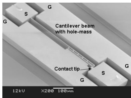
Fig. 3. SEM micrograph of a lateral switch with the hole-mass (G: ground, S: signal).
