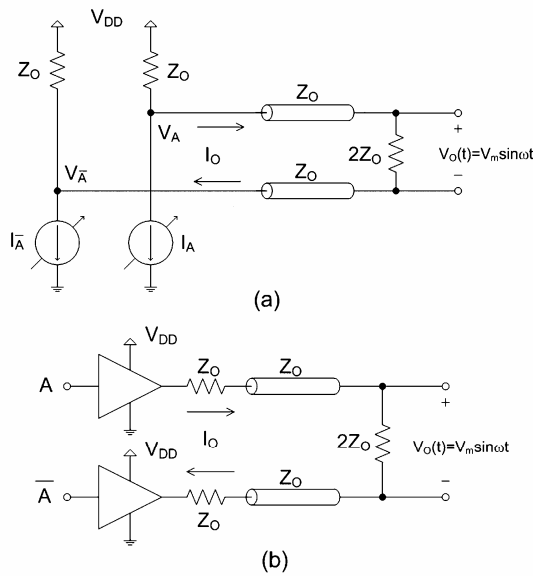
Fig. 2. Conventional (a) current-mode driver and (b) voltage-mode driver.
