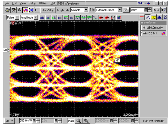
Fig. 8. Measured 5-level 1.8\text{-V}_{PP} 125\text{-MHz} eye diagram of a voltage-mode driver over 5\text{-m} UTP cable.
