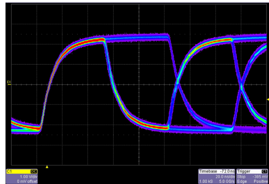
Fig. 9. Measured 4.9\text{-V}_{PP} 20\text{-MHz} waveform of a hybrid driver over 5\text{-m} UTP cable.
