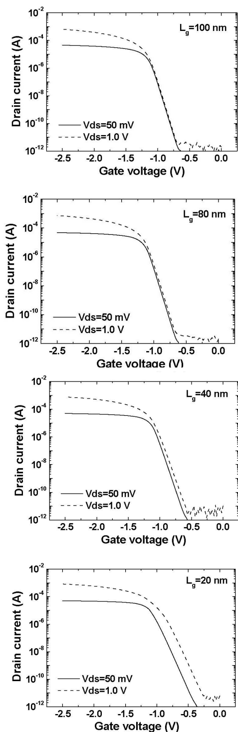
Fig. 5. I_d - V_g characteristics of p -type FinFETs fabricated by boron SPD.
