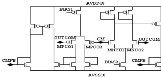
Fig. 6. Proposed static common mode feedback circuit for low voltage operation.
