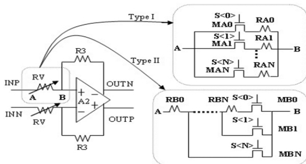
Fig. 2. The conventional PGA and resistor control.
