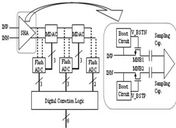
Fig. 7. The sub-sampling 6bit ADC for IF QPSK signal processing.
