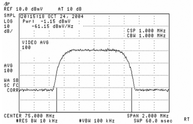
Fig. 8. The result measurement of IF QPSK receiver block.
