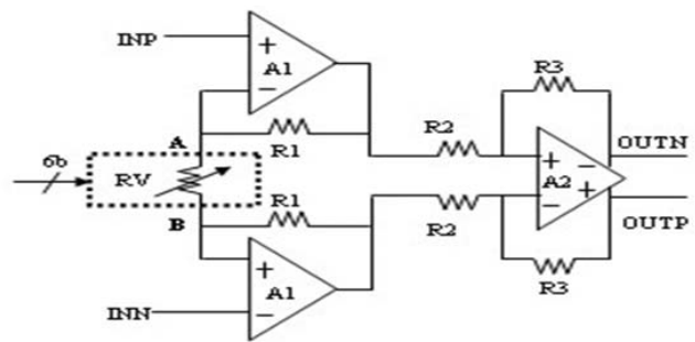
Fig. 3. The proposed PGA block.
