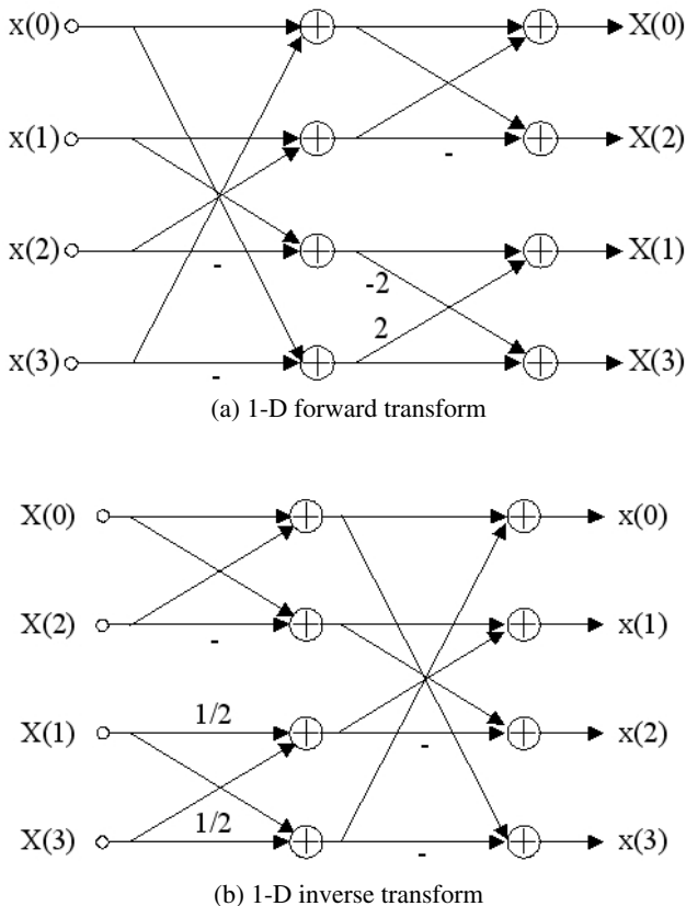
Fig. 5. Operation flow of 4 x 4 integer transform.
