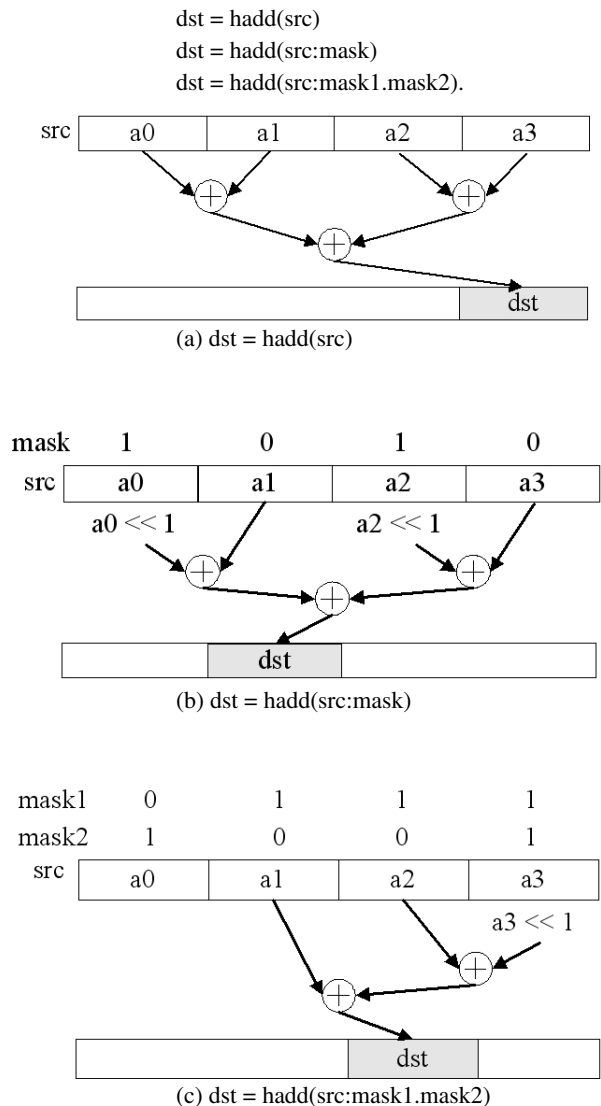
Fig. 4. Proposed instructions for packed additions within one register.
