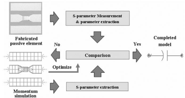
Fig. 2. Modeling flow for the passive elements.
