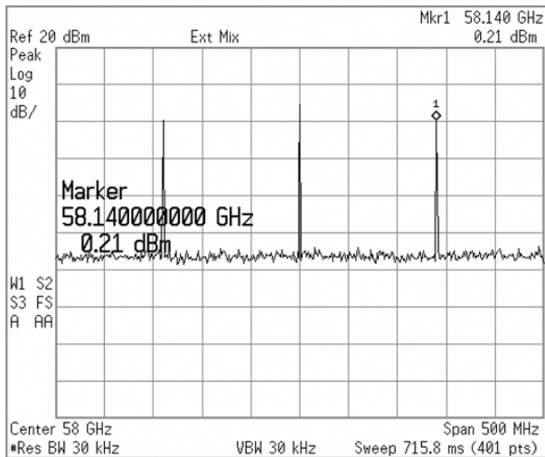
Fig. 17. Output spectrum of the V-band transmitter (IF input frequency = 140 MHz, IF input power = 0 dBm).
