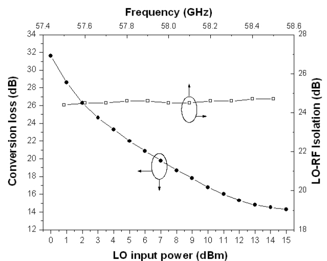
Fig. 12. Conversion loss versus LO input power, and LO-RF isolation versus frequency.
