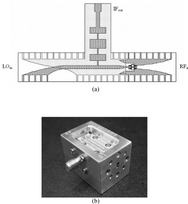
Fig. 11. (a) Layout of the designed V-band up-mixer and (b) the photograph of the up-mixer module.
