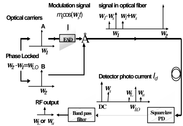
Fig. 4. Schematics of the heterodyned modulator/mixer.
