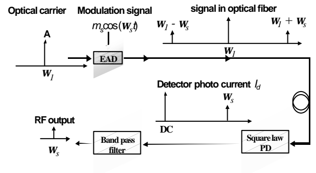
Fig. 2. Conventional RF fiber link with a single optical carrier
