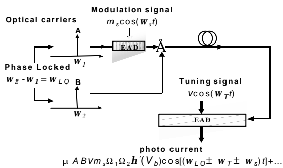
Fig. 5. RF transmission system using a modulator/mixer at the central office and a detector/mixer at the BS.
