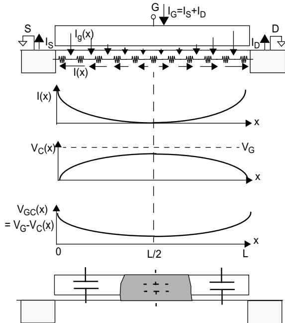
Figure 2: Current and potential distributions for a long channel MOS capacitor in the presence of gate tunneling current. Note the reduced MOS capacitor for highly leaky gate dielectrics, because of the decreased gate-to-channel bias ( V_{GC} ) near the center of the channel.
