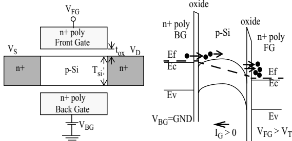
Figure 8: Cross-section of a Symmetrical DG with Ground-Plane (SGP) and corresponding band diagram for V_{FG} > V_T . tox = 1.5 nm, T_{Si} = 5-40 nm, N_{p-Si} = 1.0 \times 10^{18} \text{cm}^{-3} and N_{n-poly} = 2.0 \times 10^{20} \text{cm}^{-3} are assumed for simulation.
