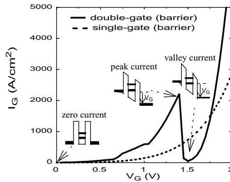
Figure 11: Simulated gate tunneling currents for double-gate (barrier) ( tox = 1.5 nm and T_{Si} = 5 nm) and single-gate MOS ( tox = 1.5 nm). Note the resonant tunneling current for double-gate structure due to the quantized energy states in the Si layer (quantum well).
