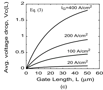
Figure 3: Current and Potential distributions in a large, leaky MOS capacitor, obtained from Eqs.(1)-(3), compared with numerical simulation using MEDICI. t_{ox}=1 nm, \rho_s=1.15K \Omega/sq. , I_0=1.33 \times 10^{-4} A/um^2 and a=0.16 , (a) current I(x) for L=50um , (b) potential V_c(x) for L=50um , (c) average voltage drop, V_c(L) with respect to gate lengths ( L ).
